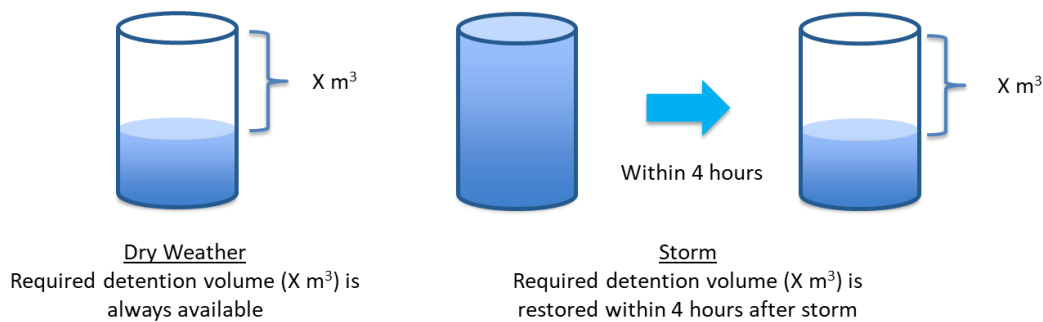
Figure 2.4.1 Schematic diagram on requirements for combined detention-rainwater harvesting systems
