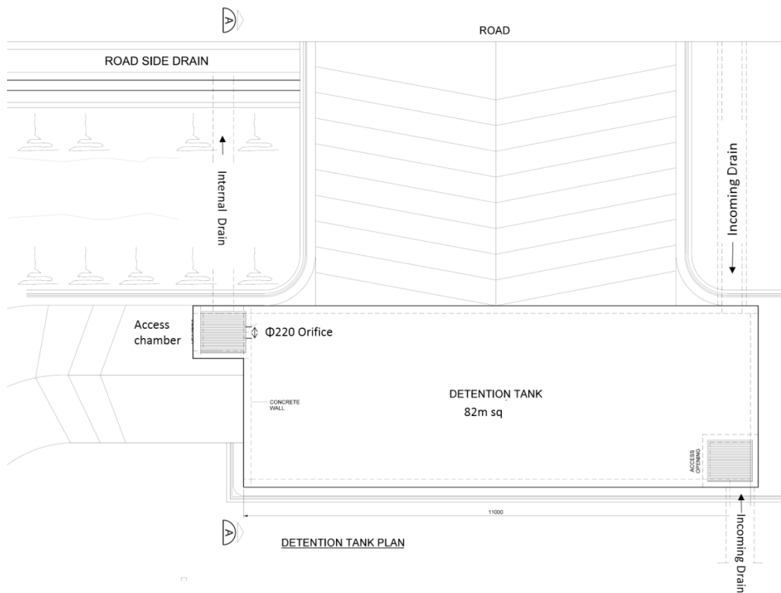
Figure 7.1.3: Detention Tank Schematic Plan
